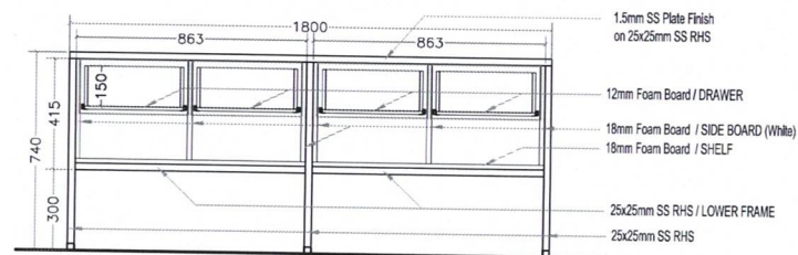
FRAME SIDE ELEVATION
