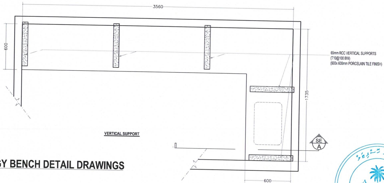
BENCH PLAN
