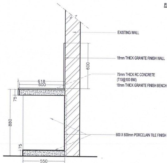
BENCH SECTION A
