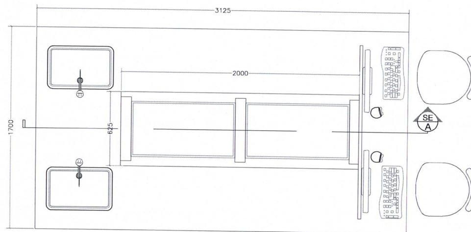
BENCH PLAN
