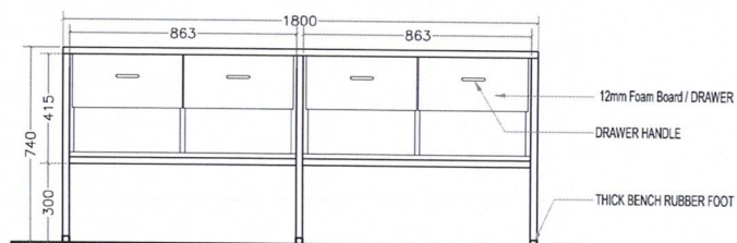
BENCH SIDE ELEVATION
