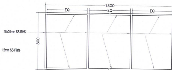
BENCH TOP FRAME
