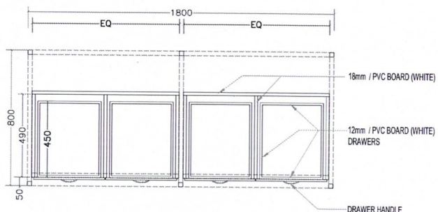
CUPBOARD FRAME PLAN
