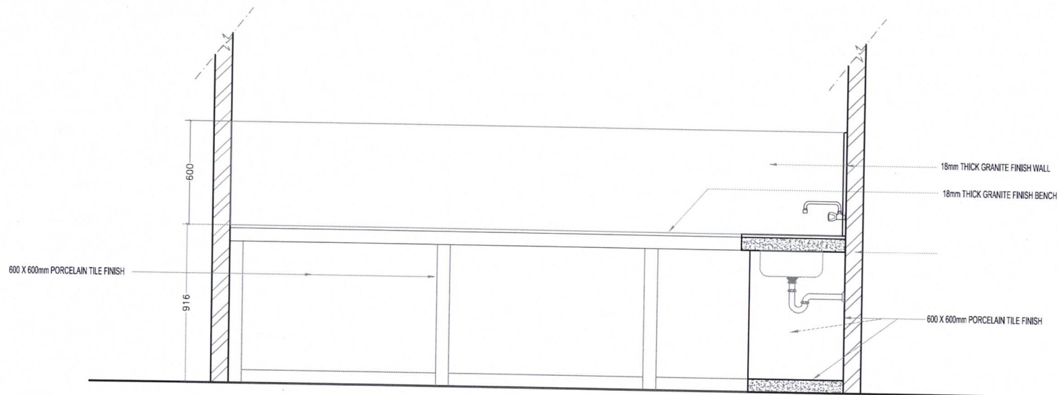
FRONT ELEVATION
