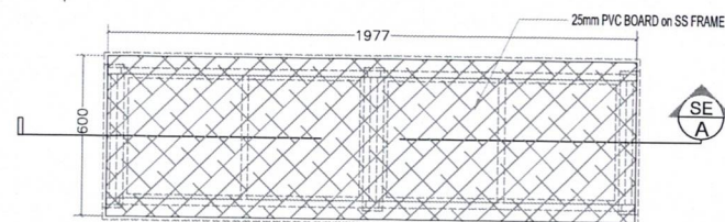
PVC BOARD
