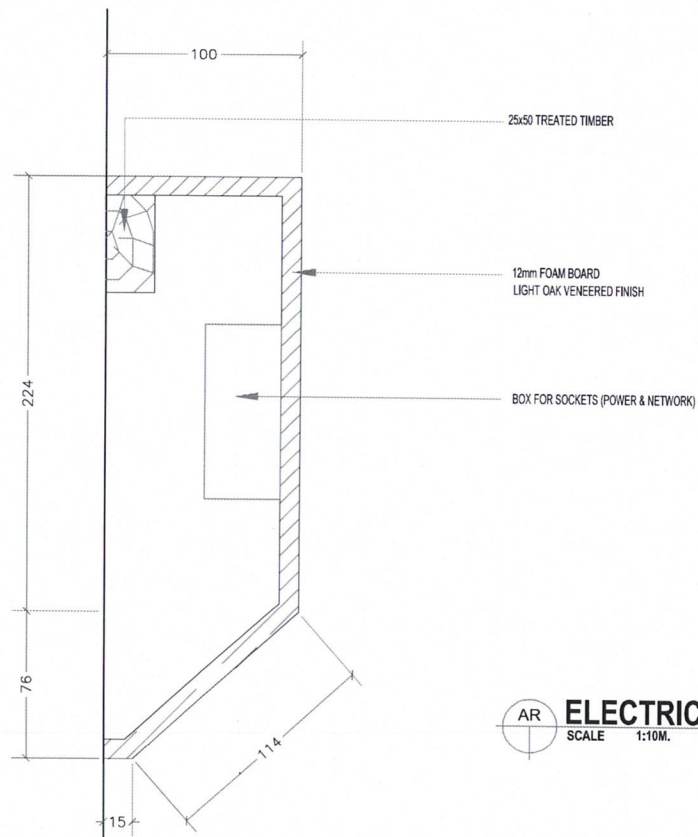
SECTION (NTS)
