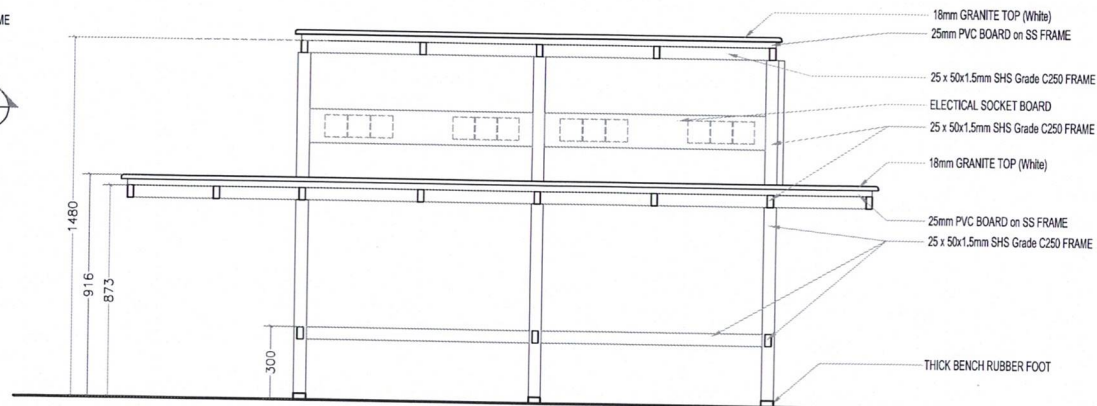
SECTION A
