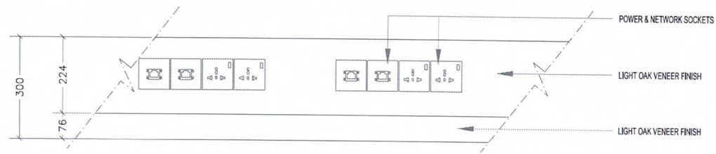
FRONT ELEVATION
