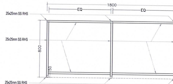
BENCH LOWER FRAME
