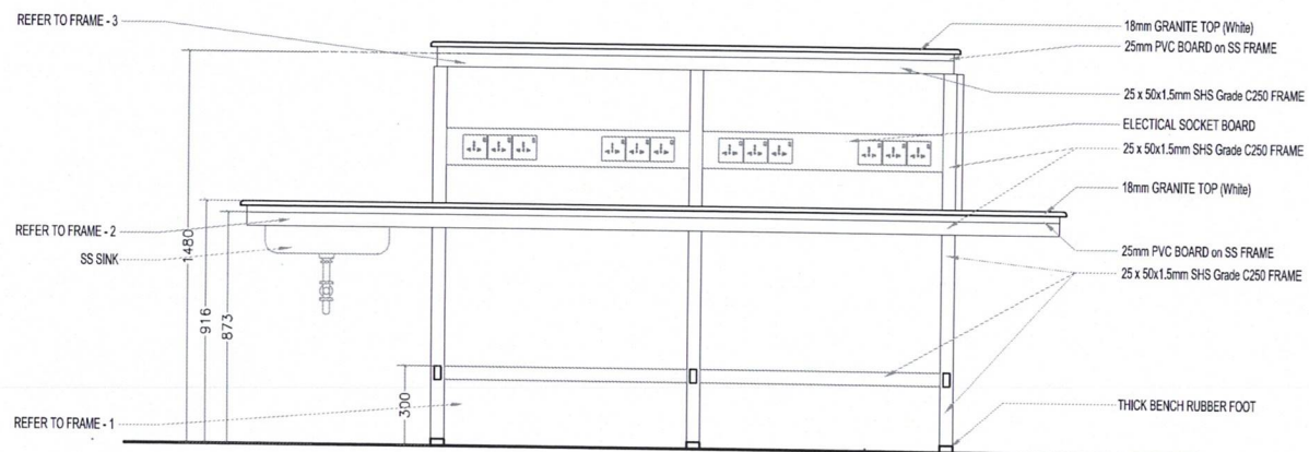
FRONT ELEVATION
