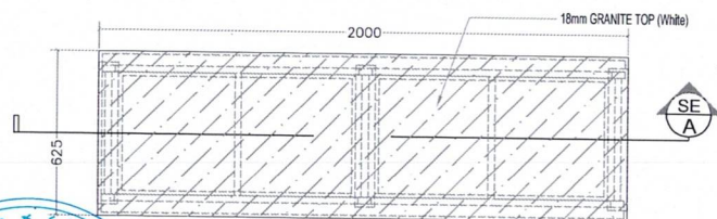
GRANITE TOP
