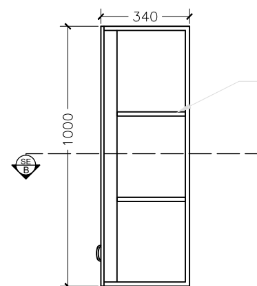
SECTION A
