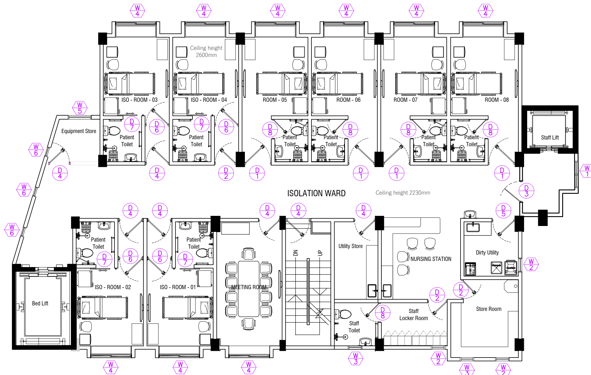
ISOLATION WARD DOOR & WINDOW REFERENCE PLAN SCALE: 1:100
