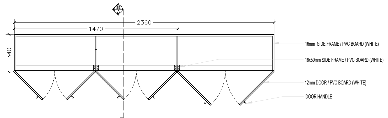
SECTION B
