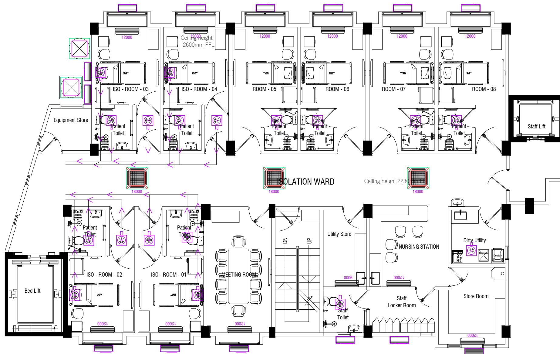
ISOLATION WARD AC & VENTILATION LAYOUT PLAN SCALE: 1:100
