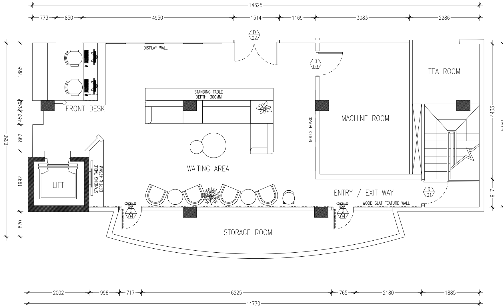
FLOOR PLAN SCALE 1:50
