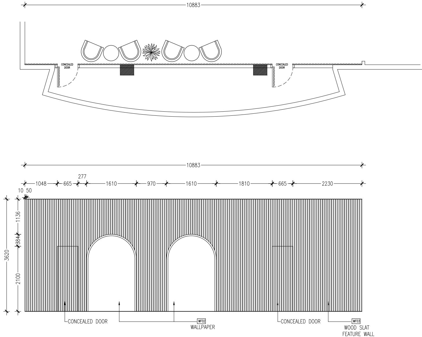
FEATURE WALL SCALE 1:50
