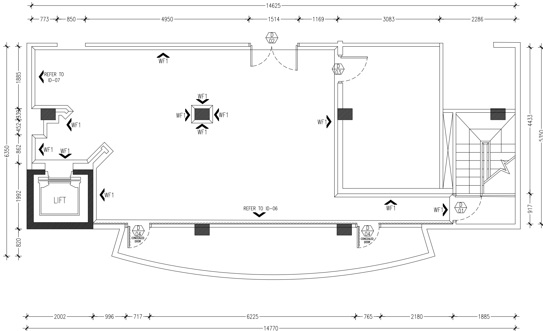
WALL FINISH PLAN SCALE 1:50
