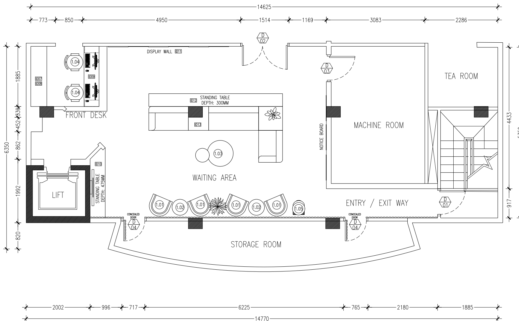
FURNITURE PLAN SCALE 1:50
