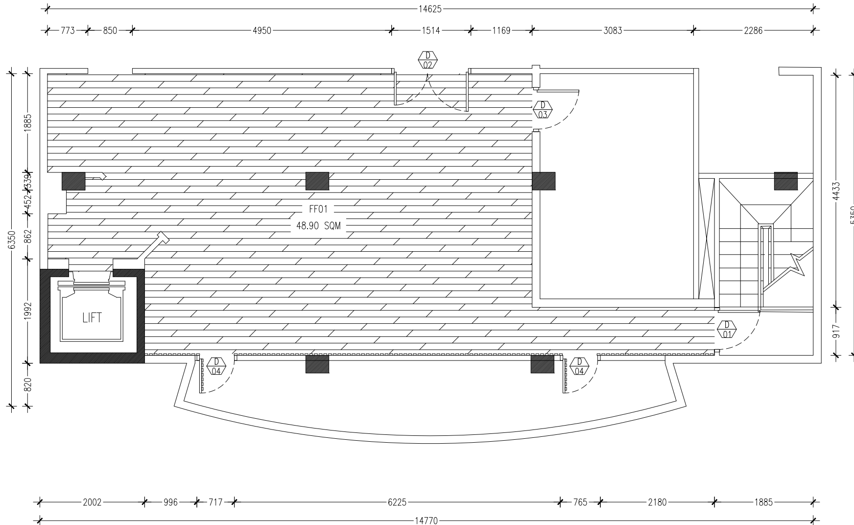
FLOOR FINISH PLAN SCALE 1:50
