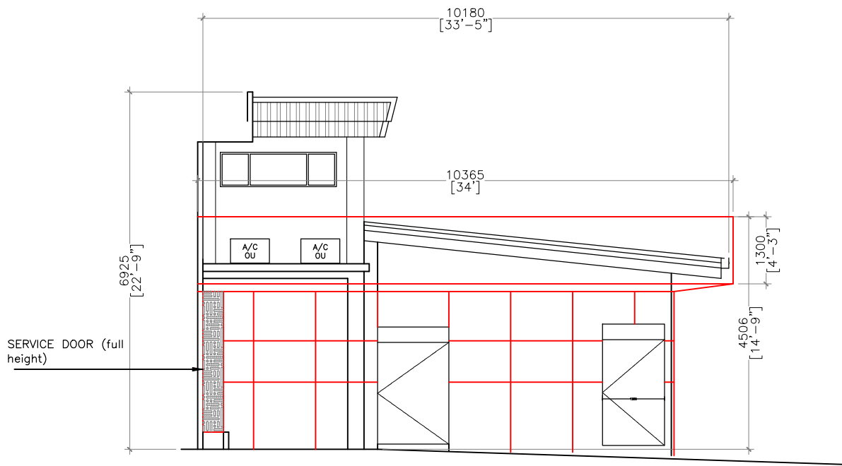
FRONT ELEVATION
