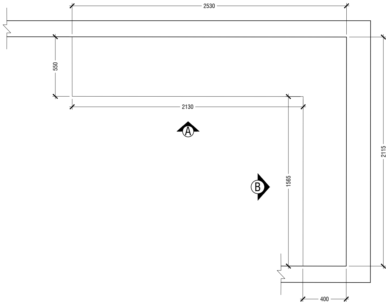
PLAN VIEW
